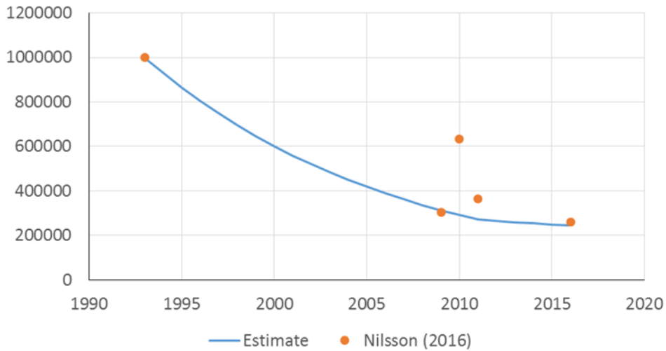
Figure 3 Counted birds on the Swedish offshore banks as reported by Nilsson (2016). The observed patterns fits a yearly population decline of 7 % until 2009 and about 2 % decline since 2011.
