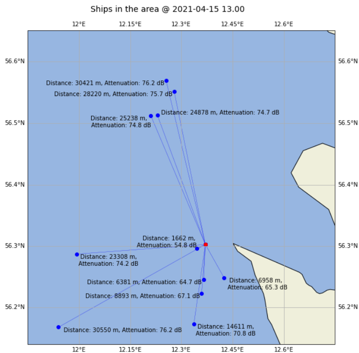
Figure 14. Top: The position of the ships (blue dots) in the sampled time slot 2021-04-15 at 13:00. The red dots show the immission points used in the calculations. Bottom: At the immission point (red), the contributions from each ship (blue) were calculated as the radiated noise minus the distance attenuation (here 17 * \log_{10}(R) , discussed below) and summarized.
